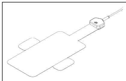
Figure 21 - Push TSMC onto Matrix
