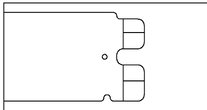
Figure 19 - Matrix connecting tail has asymmetrical cut outs, and a notch to enable correct connection
